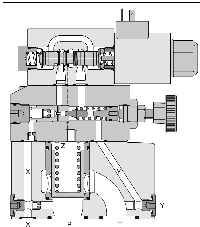
R4V06 with vent valve
